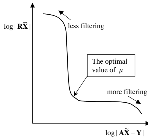
Figure 2.2: The L-curve
